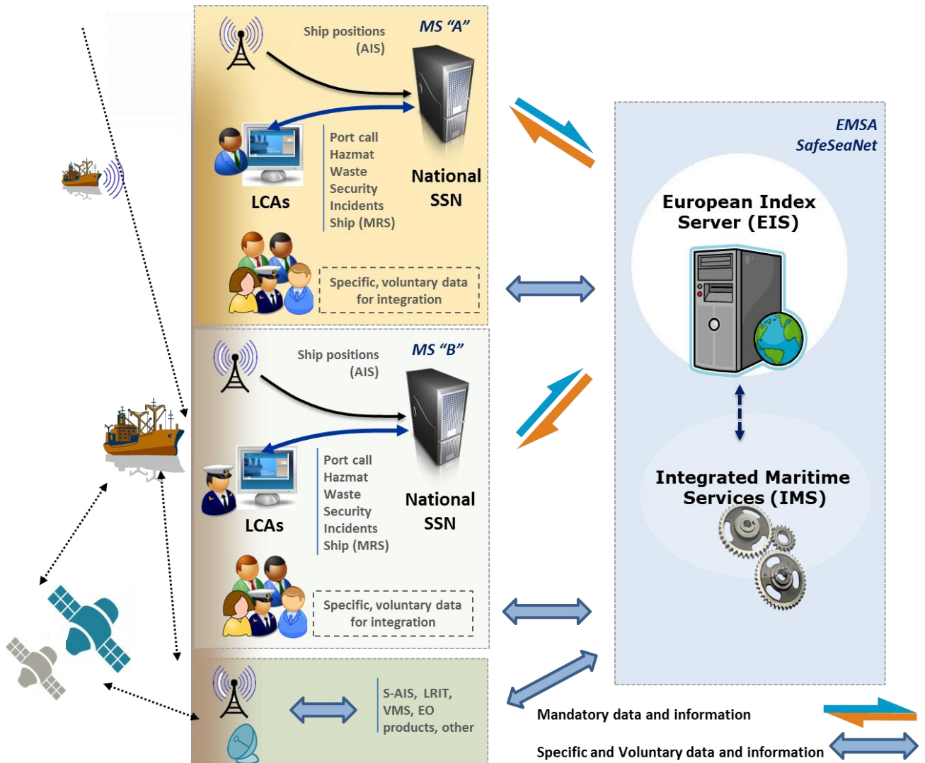
Figure 2 – SafeSeaNet system
